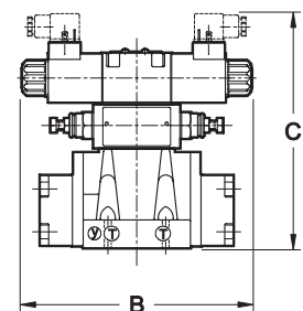
E*P4-S*/D
